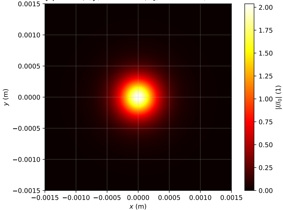
Intensity profile I(x, y, z = 1.831m)/I_0 , P_{in}=1.0P_{cr} , artificial time
